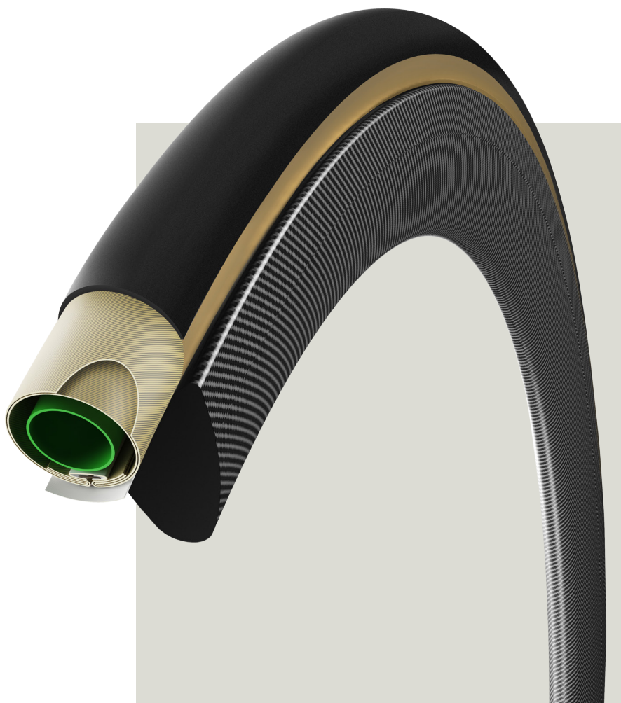
FIGURE 7. An example of tubular construction.
